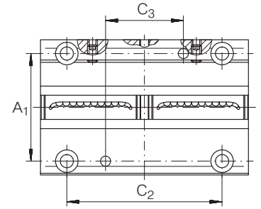
View X (rotated through 90°)
