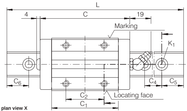
KUBE..H, plan view X (rotated through 90°)
