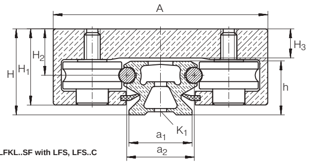
LFKL..SF with LFS, LFS..C
