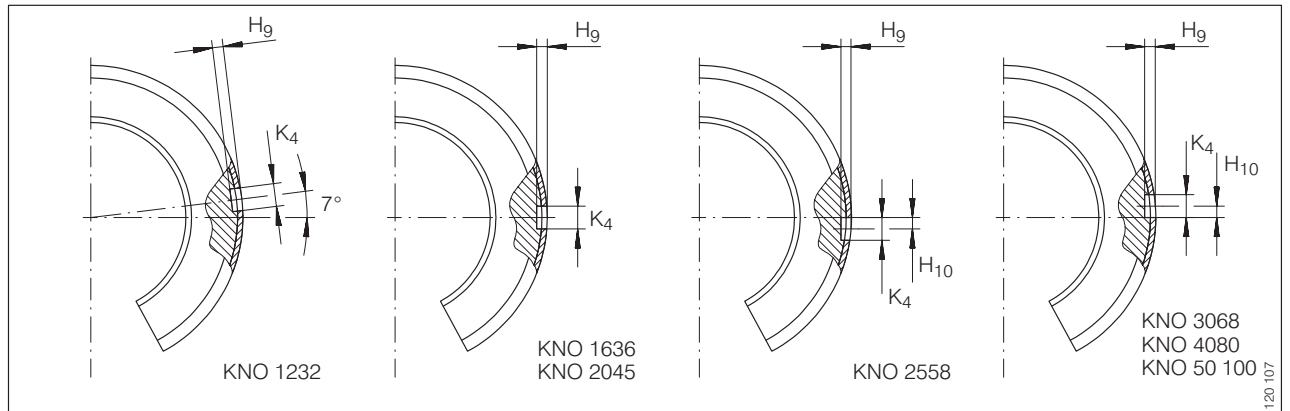
Fixing holes
