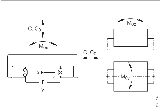
Load directions
