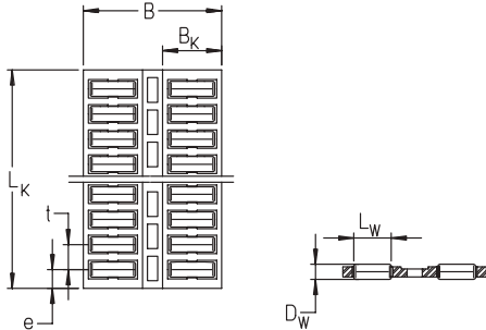
HR..ZW SERIES
