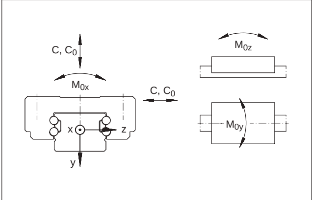
Load directions
