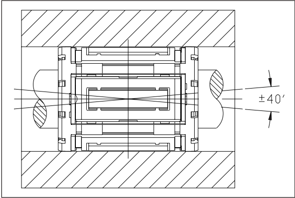
Misalignment compensation ±40'
