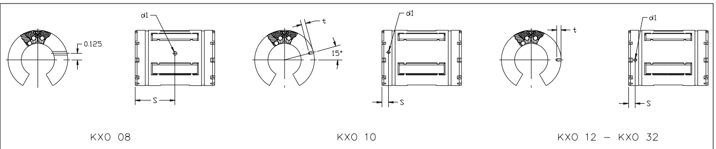
Location holes
