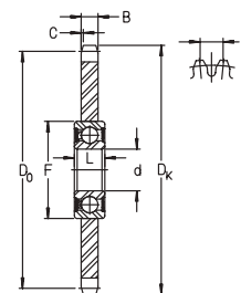
KSR..KO
