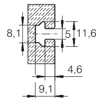
Detail X for LFS 25 M
