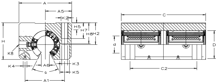
KTSO..PP AS
