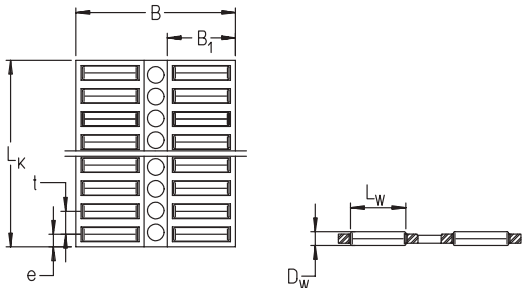
H..ZW SERIES
