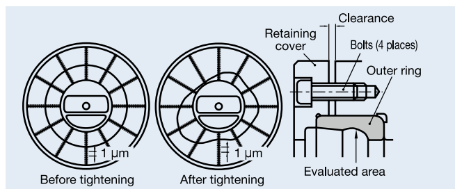
Fig. 1.19 Example of Outer Ring Deformation Caused by Tightening of Retaining Cover
