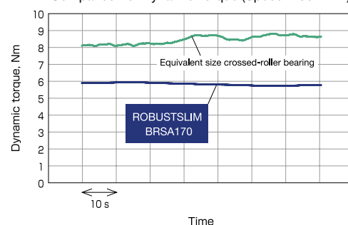
Comparison of Dynamic Torque (Speed: 100 min -1 )
