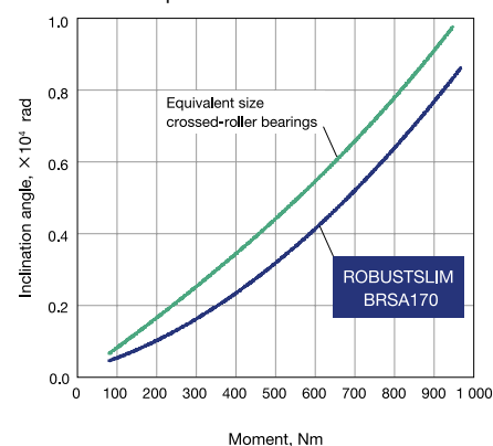
Comparison of Moment Stiffness
