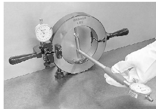
Fig. 1.9 Adjusting the GN Gauge Bore
