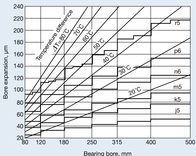
Fig 1.25 Temperature and Thermal Expansion of Inner Ring
